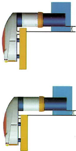
Fig 17-1 Fig 17-2 7.2 Tools needed: percussive drill, dia.8mm; cross screwdriver, dia.6mm.
